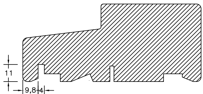
4mm zinknot
